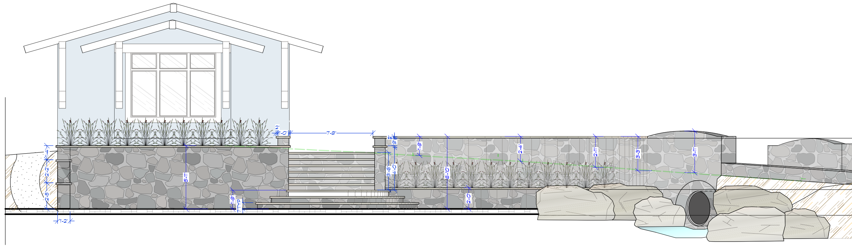
1 Front Garden Elevation - As Built Scale: 3/16" = 1'-0"
